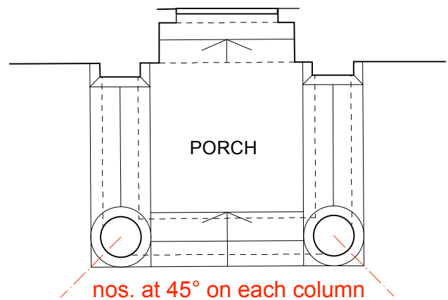
PROJECTING PORCHES
